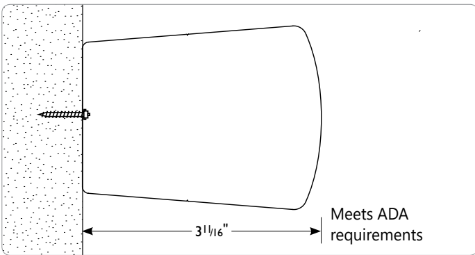
SIDE DETAIL
