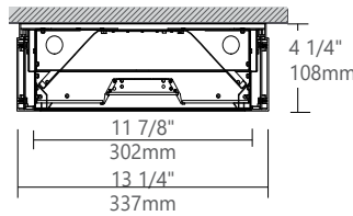
SECTION VIEW
