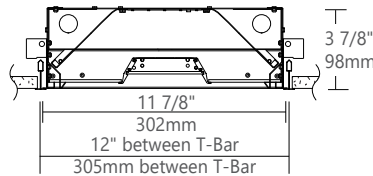
SECTION VIEW
