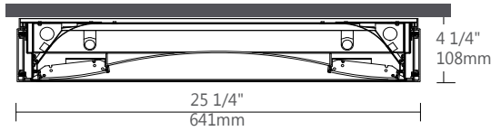
SECTION VIEW
