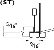
SCREW SLOT
