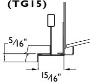
15/16" TEGULAR
