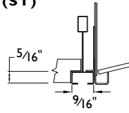
SCREW SLOT
