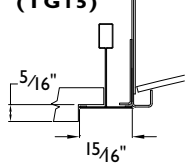
15/16" TEGULAR
