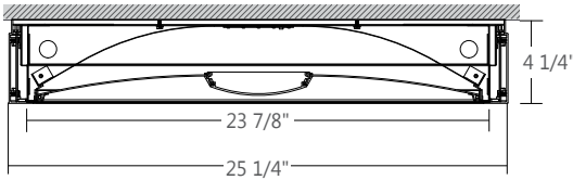
SECTION VIEW
