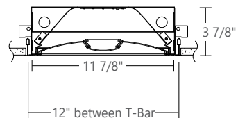
SECTION VIEW
