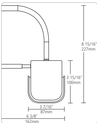
MOUNTING BRACKET
